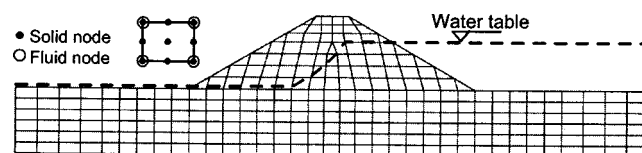
Fig. 3. Finite element mesh and employed solid–fluid coupled element
